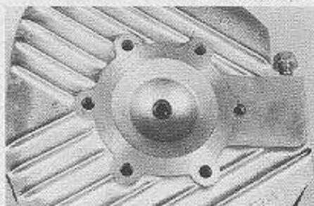
The KX's cast aluminum head has a concentric shaped combustion dome with a wider-than-usual squish band.
