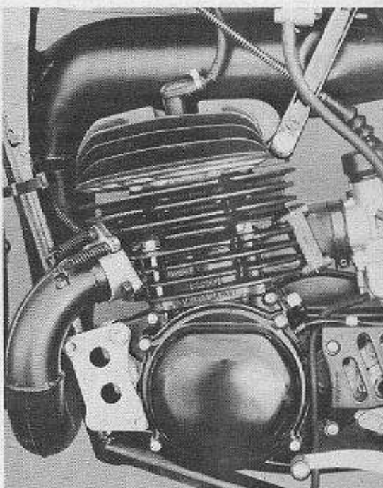
Head stay serves as an additional engine mount to increase frame rigidity; it also helps mute vibrations.
