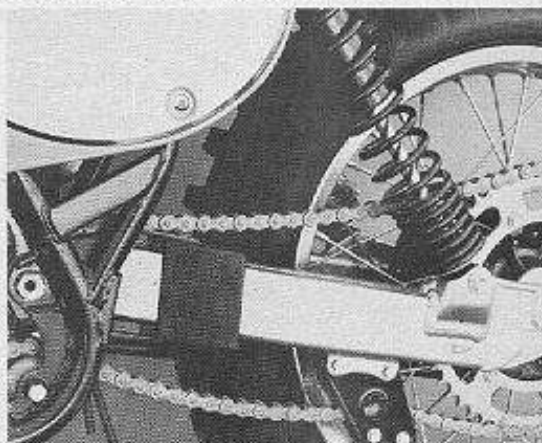
Stout aluminum box-section swing arm has an I-beam rear section, hollow swing-arm pivot bolt and axle.
